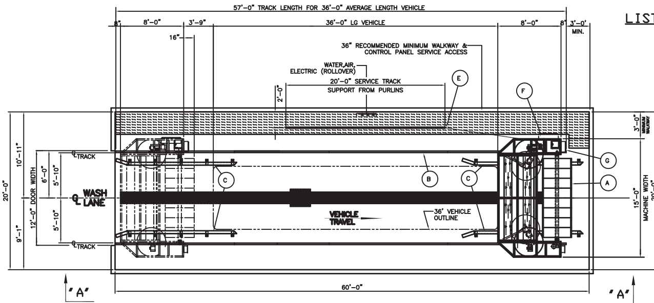
PLAN VIEW LAYOUT OF EQUIPMENT MODEL #T-126 ROLLOVER WASHER
