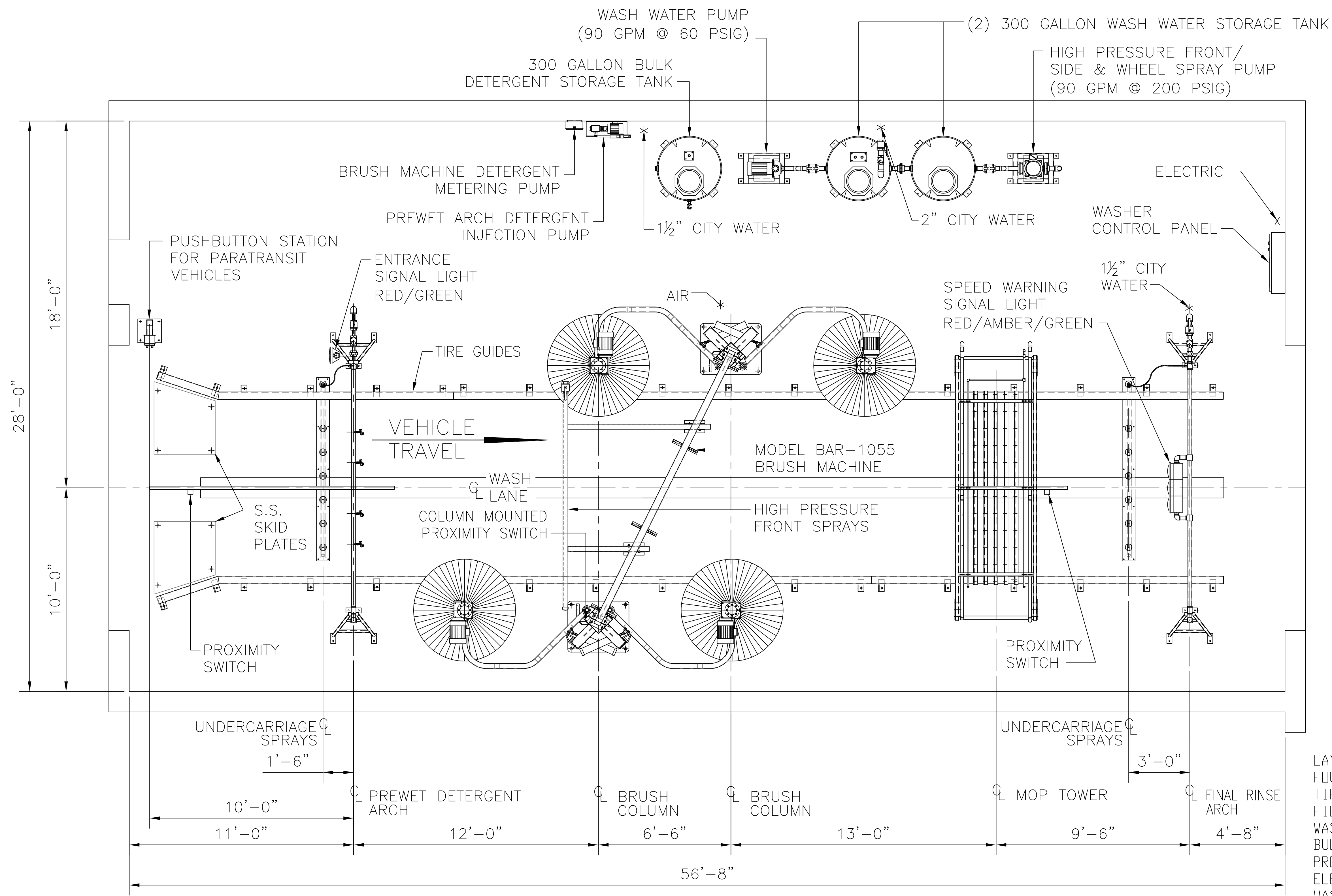
PLAN VIEW LAYOUT OF EQUIPMENT
