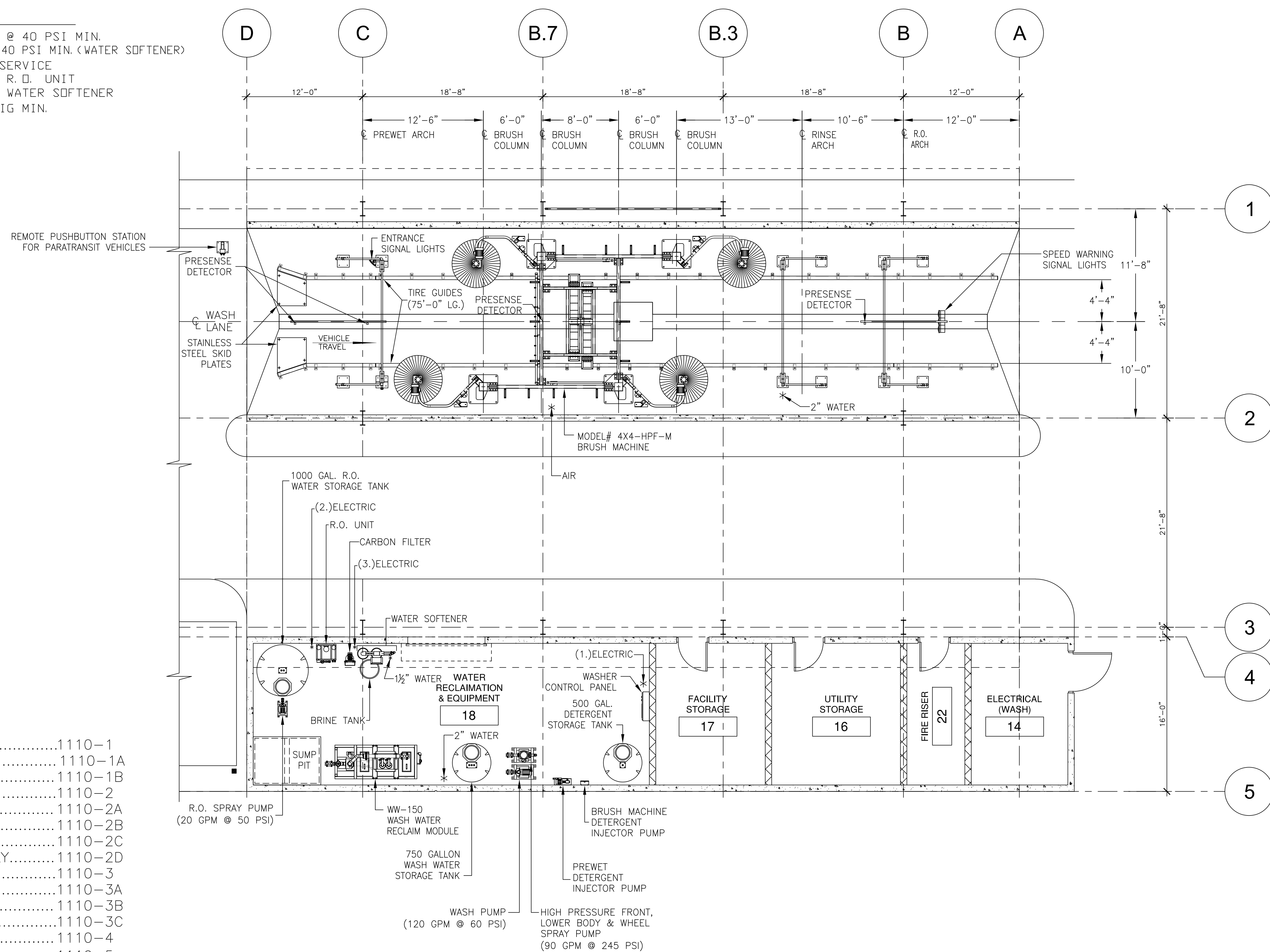
PLAN VIEW LAYOUT OF EQUIPMENT
