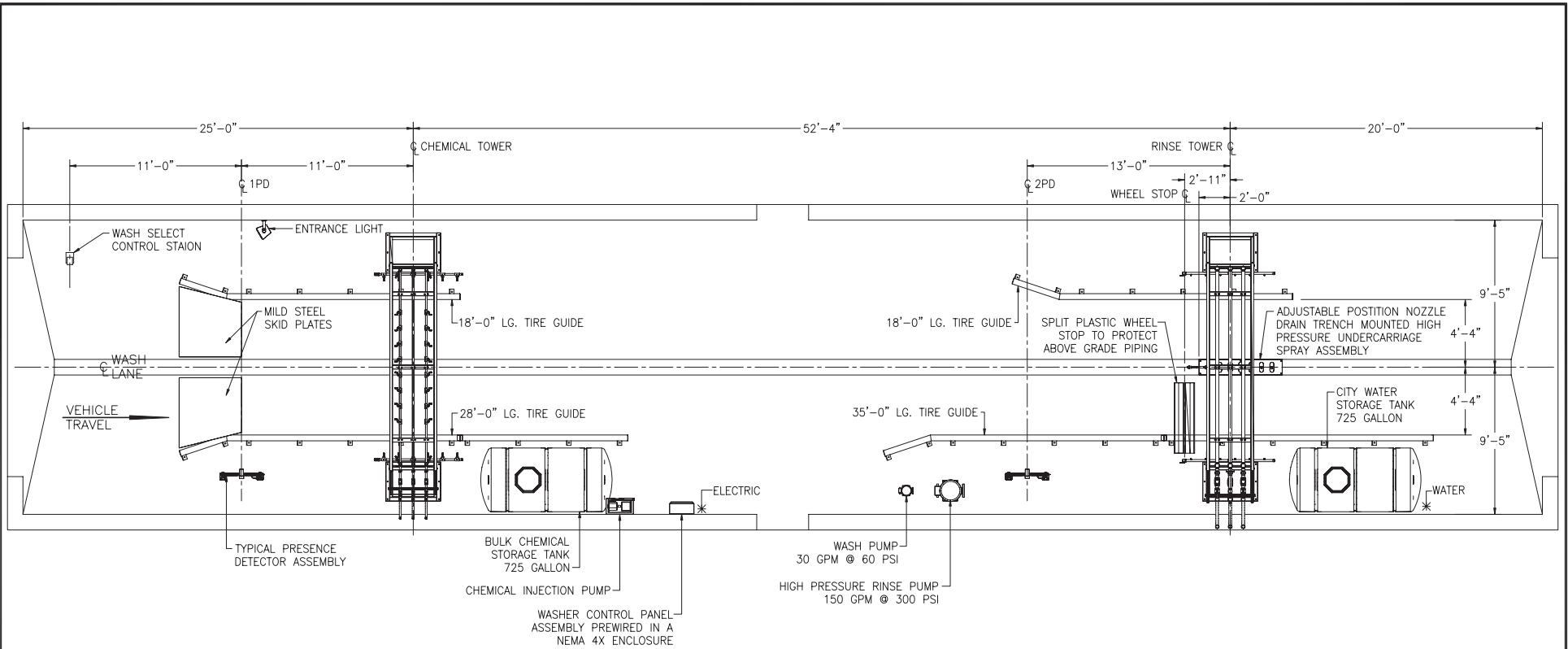
PLAN VIEW LAYOUT OF EQUIPMENT
